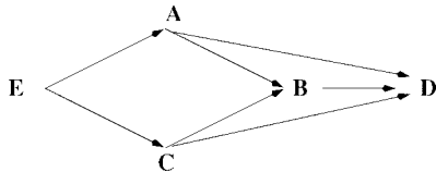
Fig. 7. A datum flow chain for the assembly of Fig. 2.
